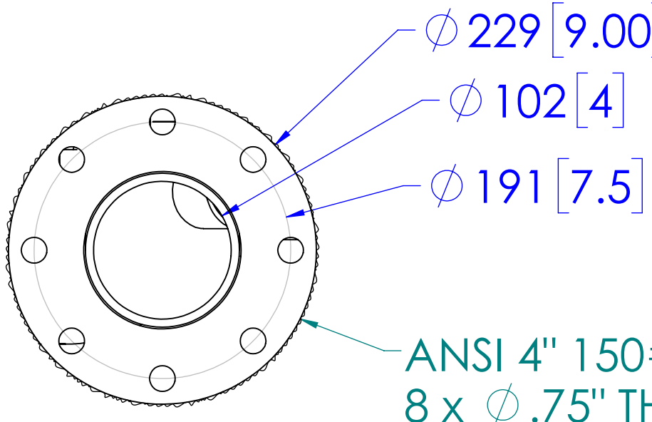
DETAIL A OPTIONAL DRY EXHAUST FLANGE SCALE 1 : 4
