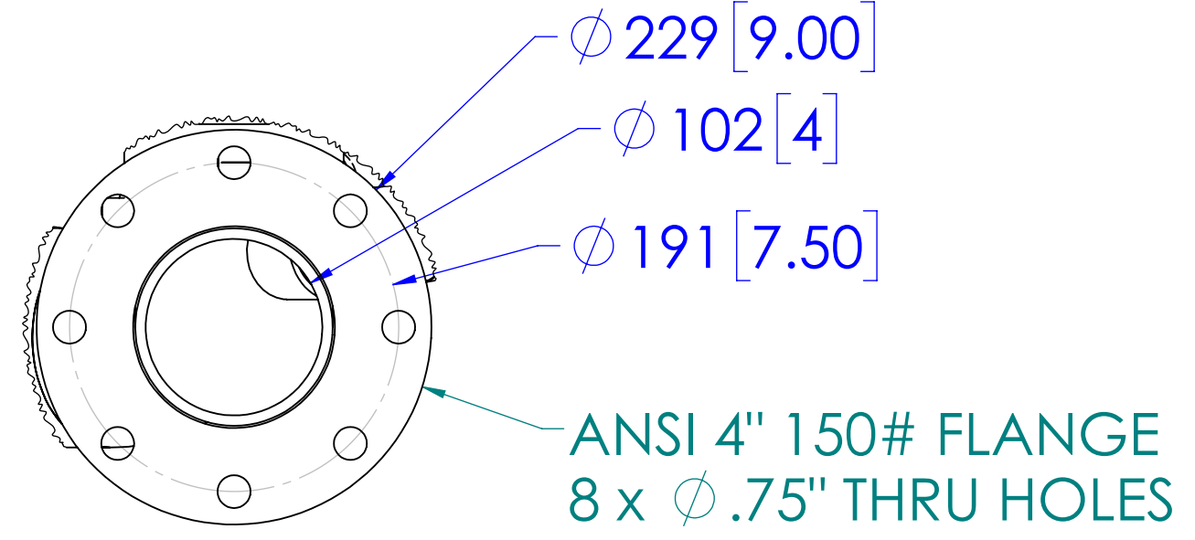
DETAIL A OPTIONAL DRY EXHAUST FLANGE SCALE 1 : 4
