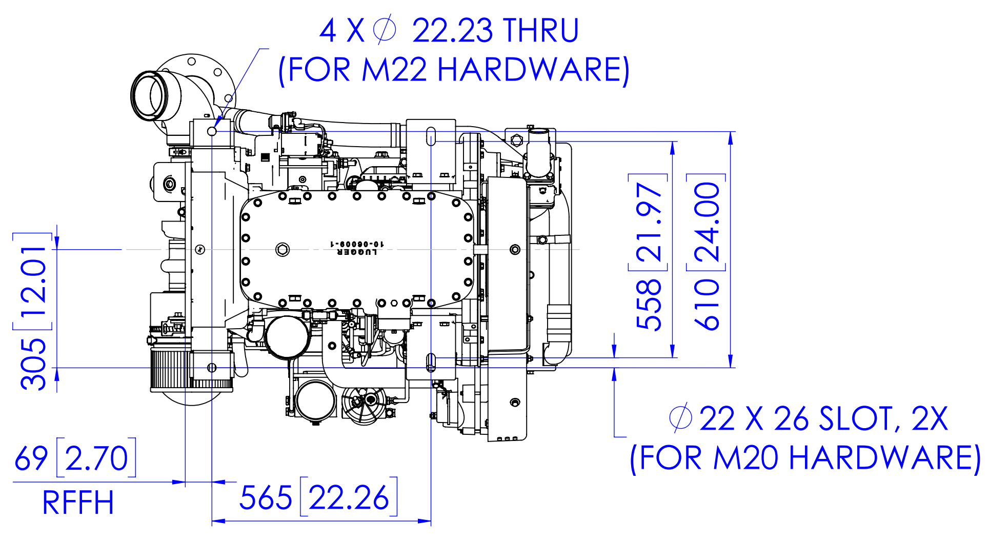
MOUNTING (W/O VIBRATION ISOLATION)
