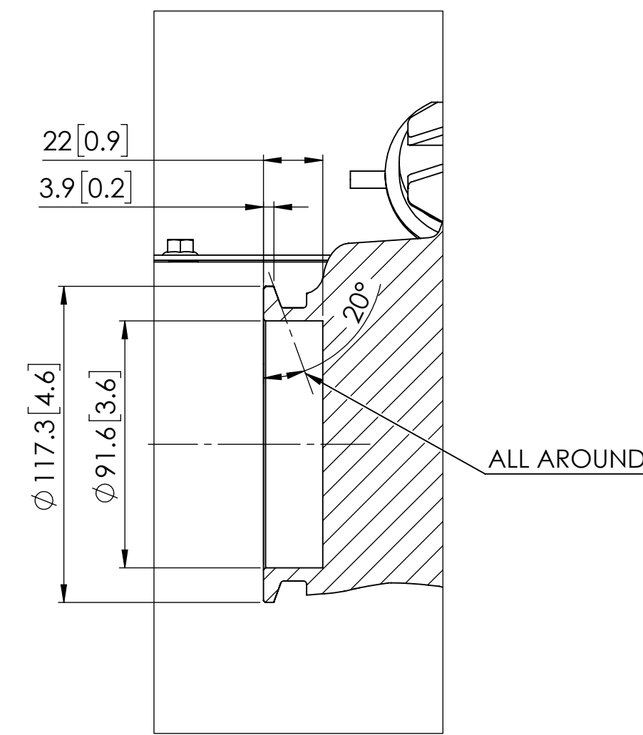
SECTION B-B SCALE 1 : 2 EXHAUST CONNECTION DIMENSIONS
