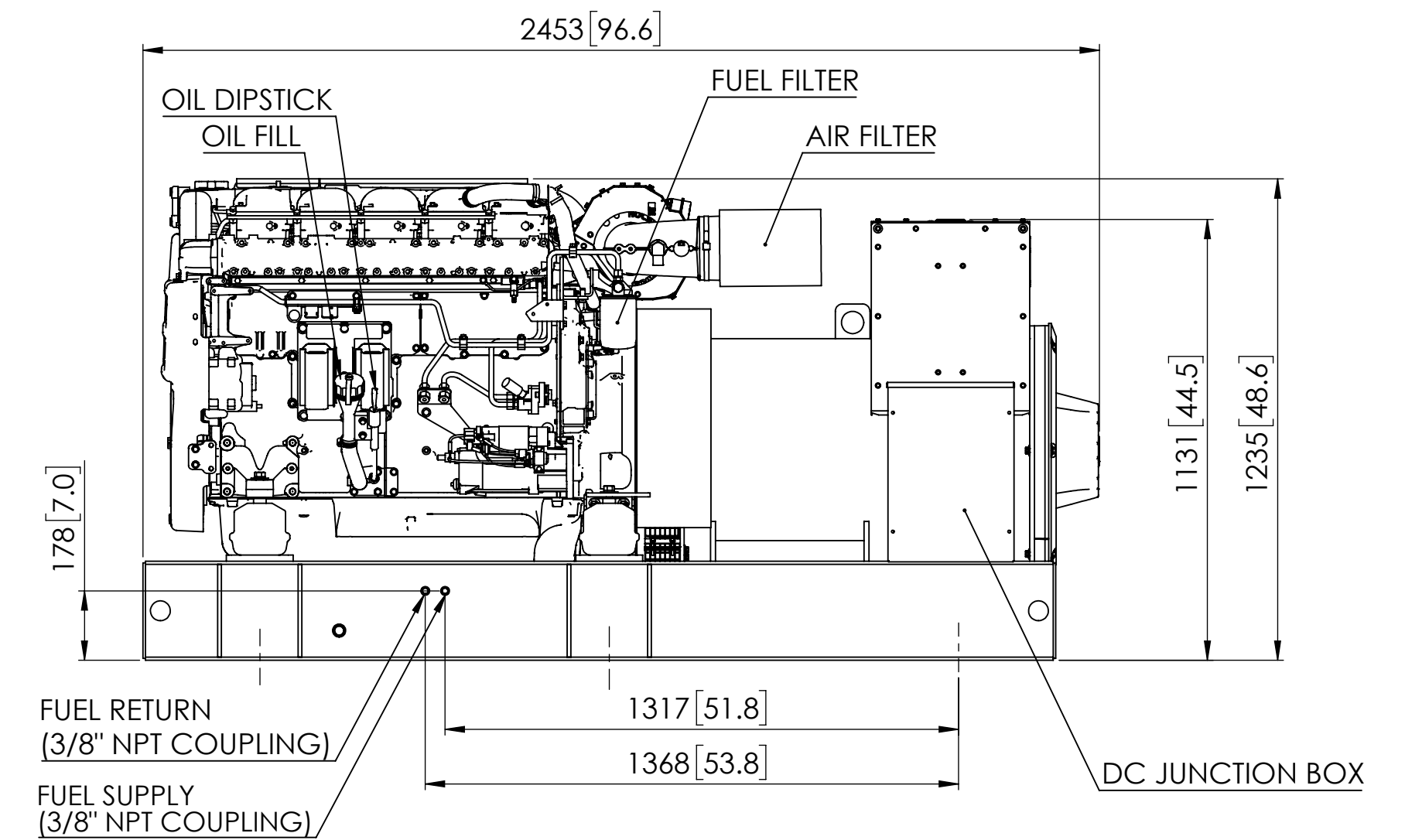
RIGHT (SERVICE) SIDE VIEW
